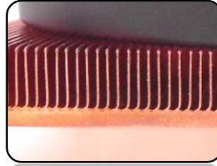
All copper, Skive Fin Technology
